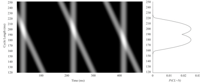
Figure 3: (Left) Time vs CL map on a 500ms time window. (Right) MI curve extracted from the map. The two local maxima correspond to the two values of CLs of the signal: 180 ms and 200 ms.
